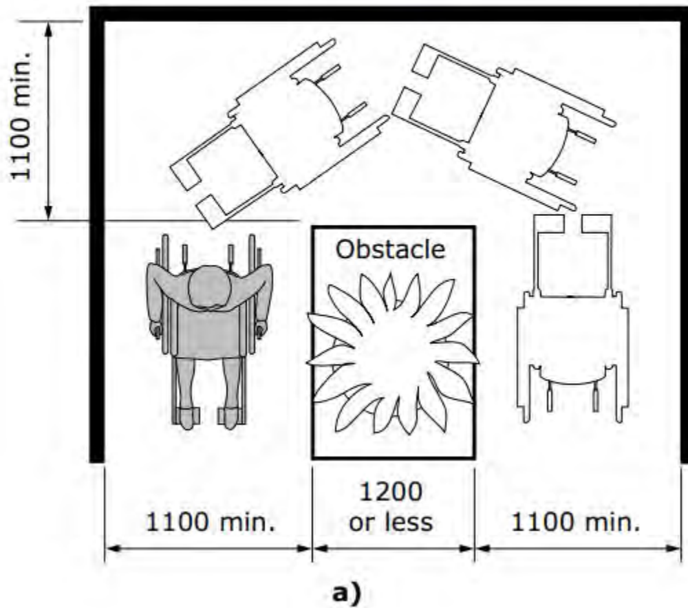
Figure 16 Width of accessible route around an obstacle (See Clause 5.1.1.)
